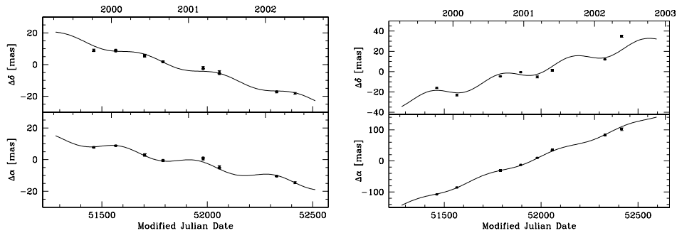
Figure 2. For S CrB (1667 & 1665; left) and R Cas (1665; right) only spots in the receding part of the shell could be found. Still, satisfying fits of proper motion and parallax could be made, especially for S CrB which has the closest reference source.
