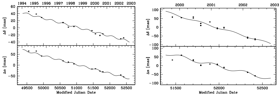
Figure 1. The position of the most blue-shifted 1667 MHz maser spot of U Her (left) with respect to the reference source, spanning approximately 8 years. For W Hya (right) both 1665 and 1667 blue-shifted spots are used. Note that the observations only span 2.5 years. The drawn line represents the best fit for proper motion and parallax.
